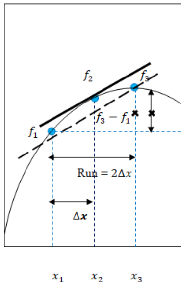
Fig. 1: Centre Difference Technique Presented at a point f_2
