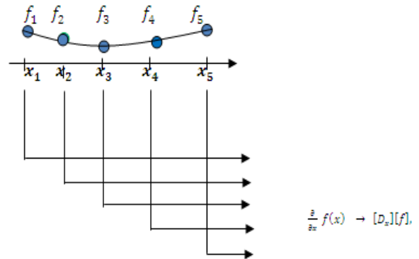
Fig. 2: The derivative of a function geometrically presented at any prescribed point
