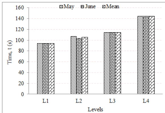
Fig. 4: Time elapsed for filling up of water tank at selected levels
