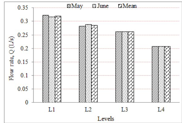
Fig. 5: Flow rate at selected levels
