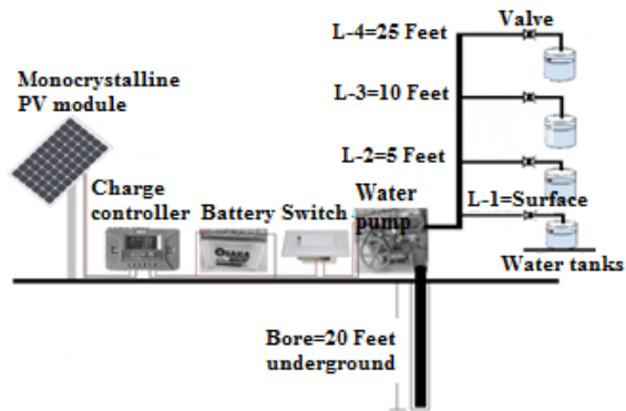
Fig. 1: Schematic diagram of installed water pumping system
