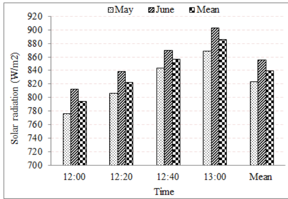
Fig. 2: Global solar radiations during experimental work
